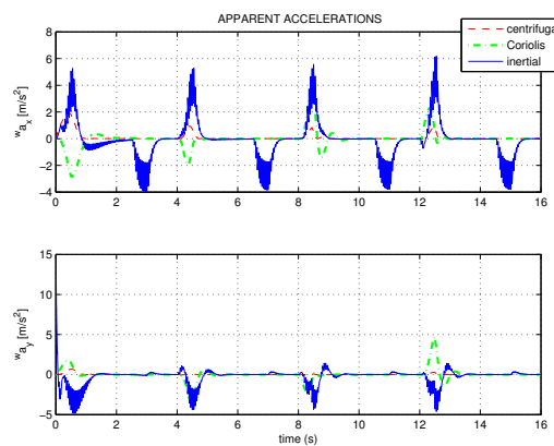
Fig. 8. Inertial, centrifugal and Coriolis components of the apparent acceleration felt by the user in the X_w (top) and Y_w (bottom) directions, due to the carpet accelerations of Fig. 6
